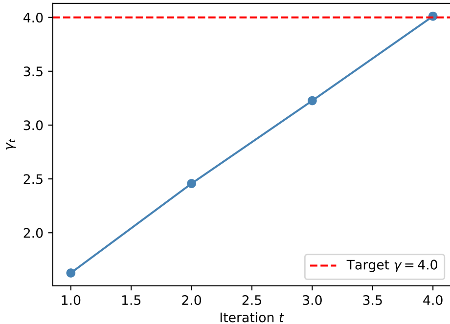
CE Method: Level sequence \gamma_t
