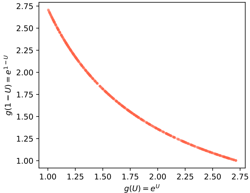
Payoff pairs (\rho = -0.968)
