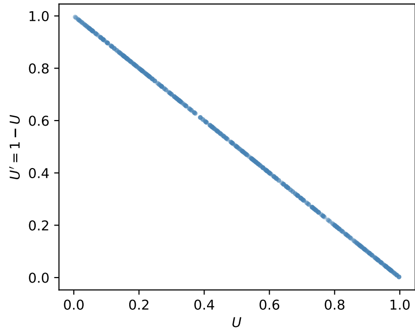
Antithetic pair (U, 1 - U)
