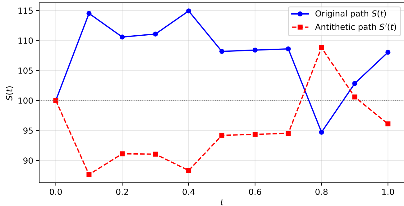
Asian Option: Original vs Antithetic Paths ( n = 10 )
