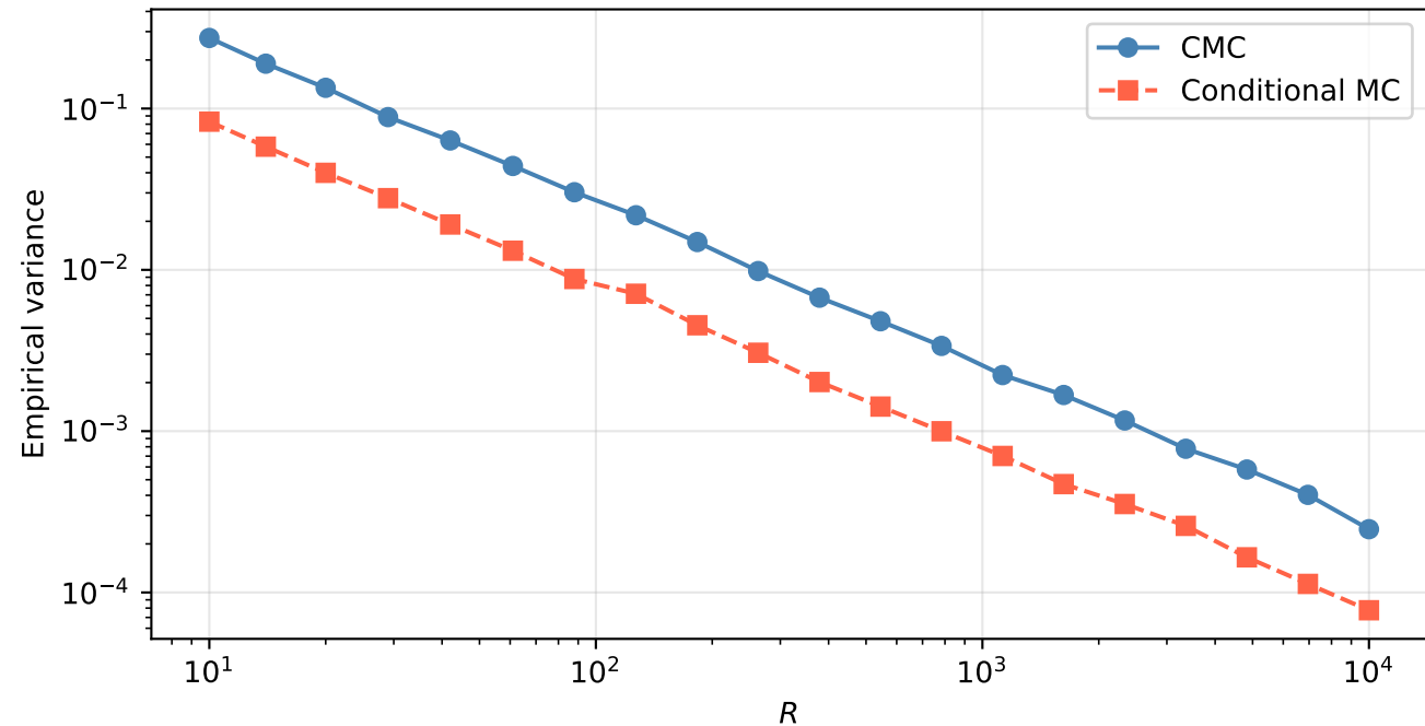
Conditional MC vs CMC for \pi estimation
