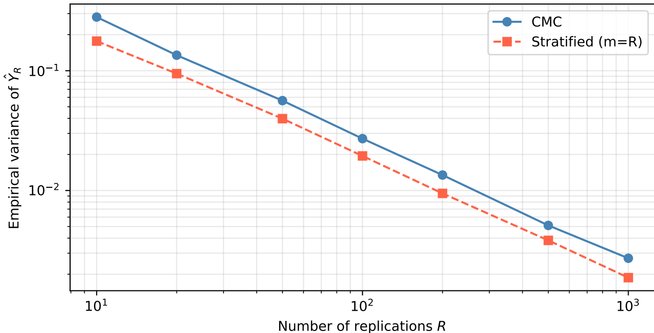
Variance Comparison: CMC vs Stratified Sampling ( \pi estimation)
