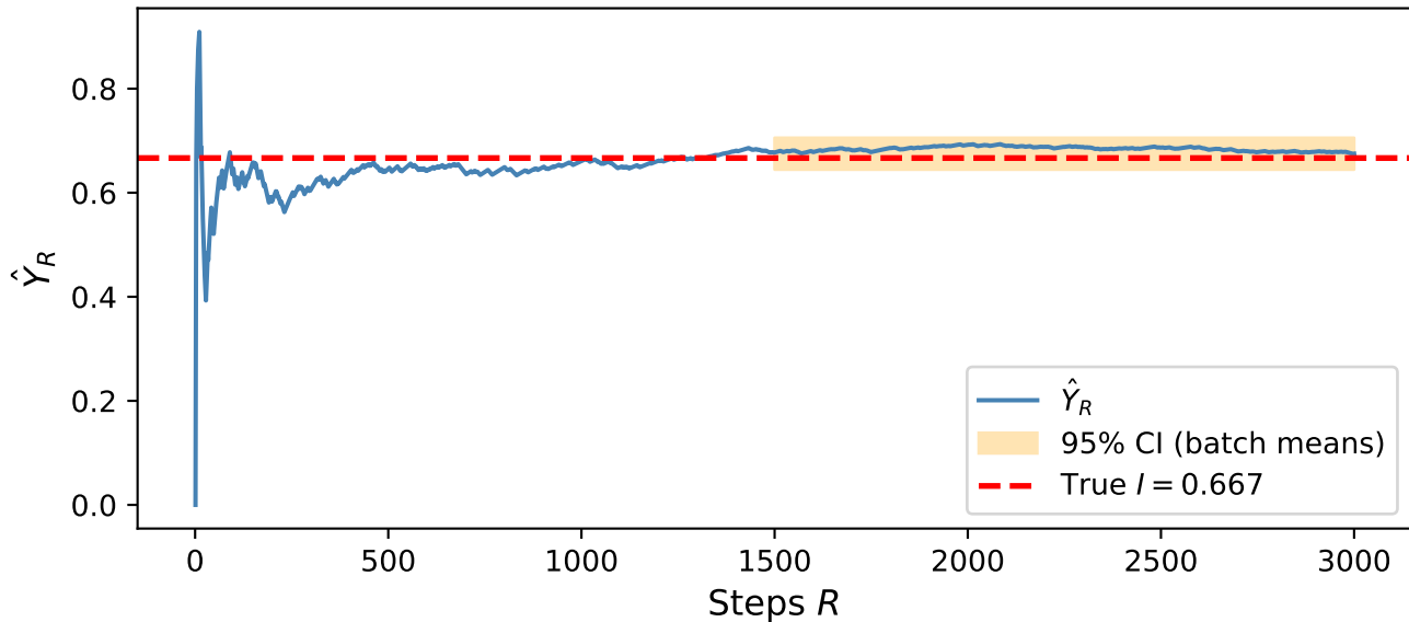
MCMC estimator with batch means confidence interval
