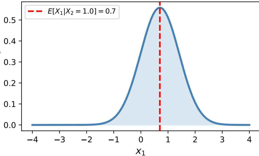
Full conditional p(x_1|x_2 = 1.0) (bivariate normal, \rho = 0.7 )
