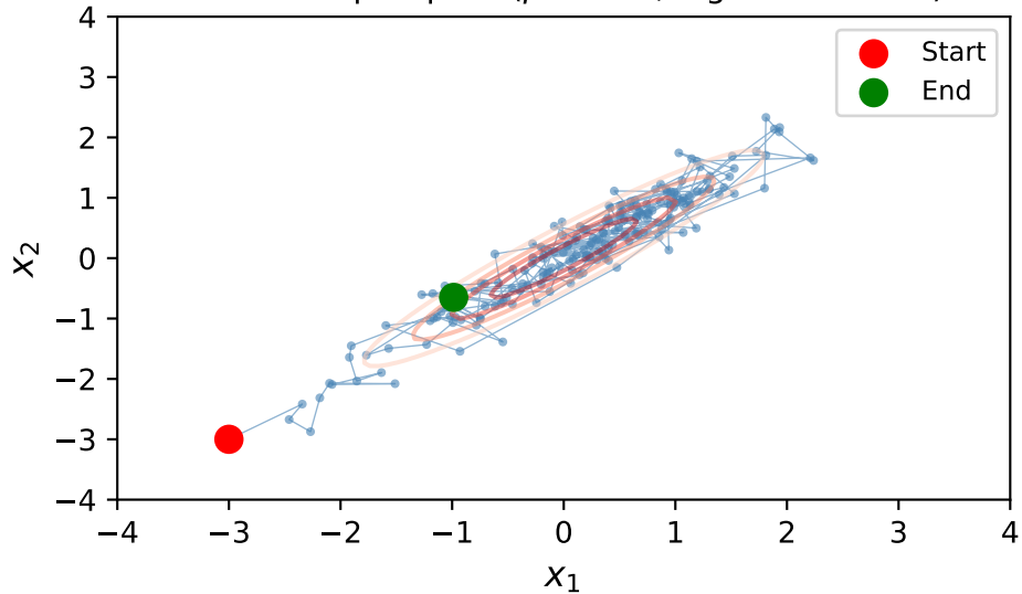
Gibbs sampler path ( \rho = 0.95 , high correlation)
