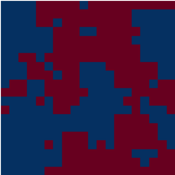
Ising model sample ( \beta = 0.45 , 20x20 grid)
