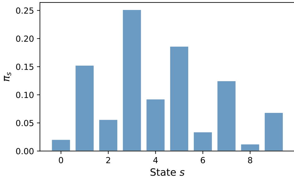
Target distribution \pi
