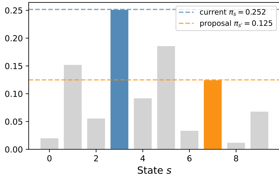
Acceptance ratio \alpha = \min(1, \pi_{s'}/\pi_s) = 0.497
