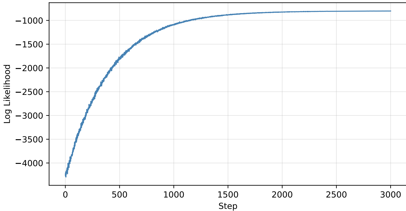
Fig 7.1 - Metropolis for substitution cipher: log-likelihood
