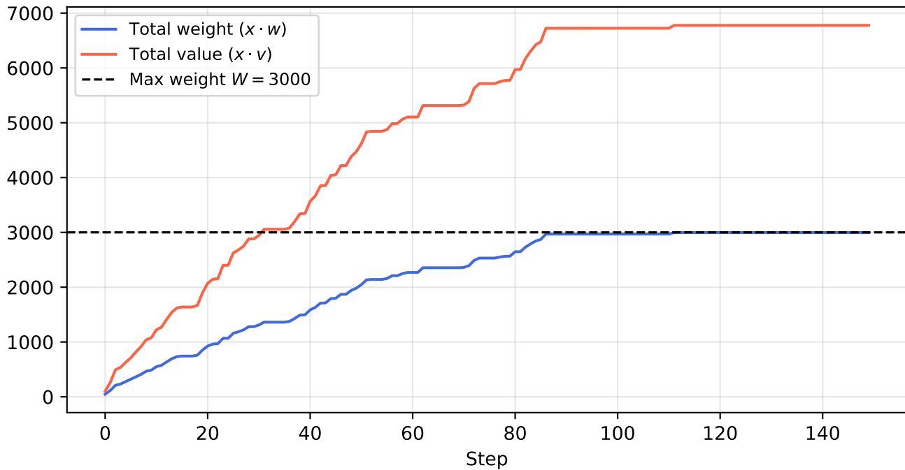
Fig 7.2 - Knapsack (Metropolis, d = 100 , W = 3000 )
