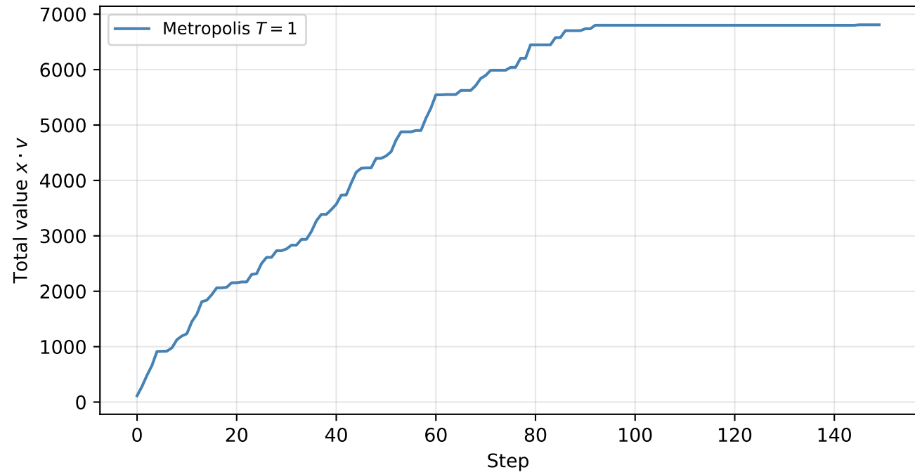
Knapsack - Metropolis algorithm ( d = 100 , W = 3000 )
