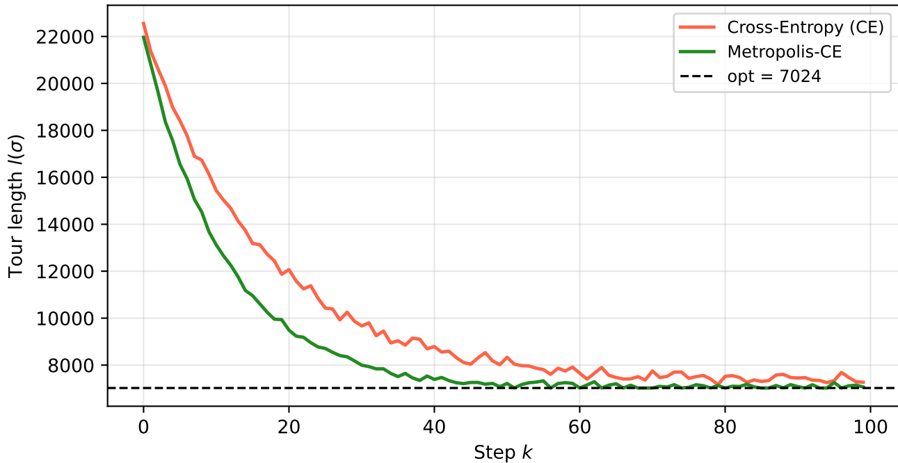
Fig 7.5 - Metropolis-CE vs CE on TSP (13 cities)
