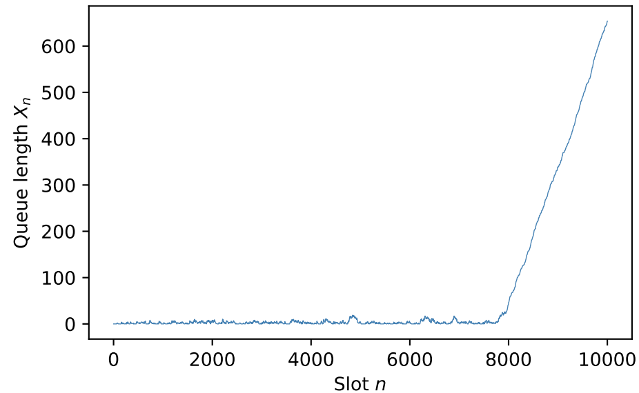
Slotted ALOHA: \lambda = 0.31 , h = 0.1
