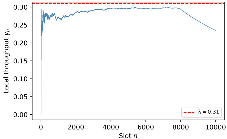
Local Throughput
