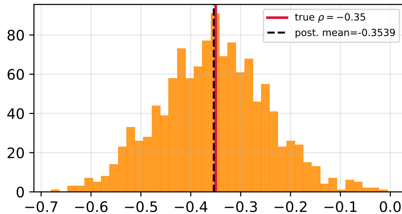
HMC posterior: \rho
