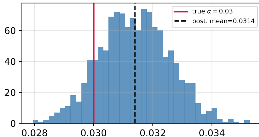
HMC posterior: \alpha
