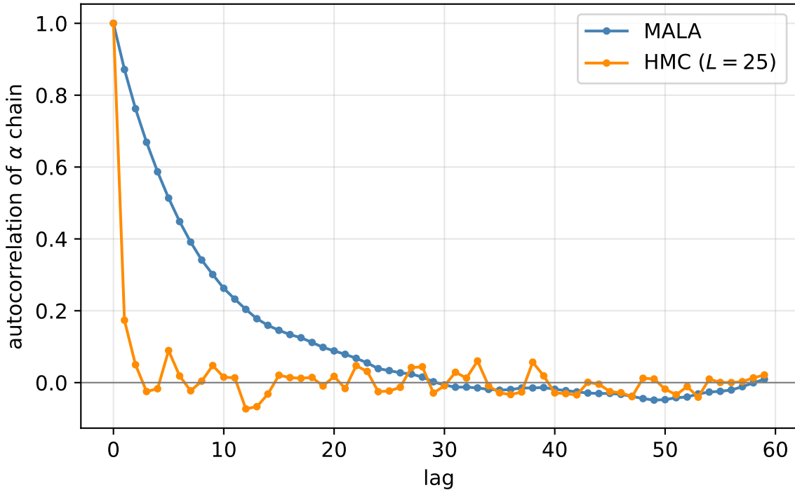
Toy example: HMC mixes faster than MALA (autocorrelation decays quicker)
