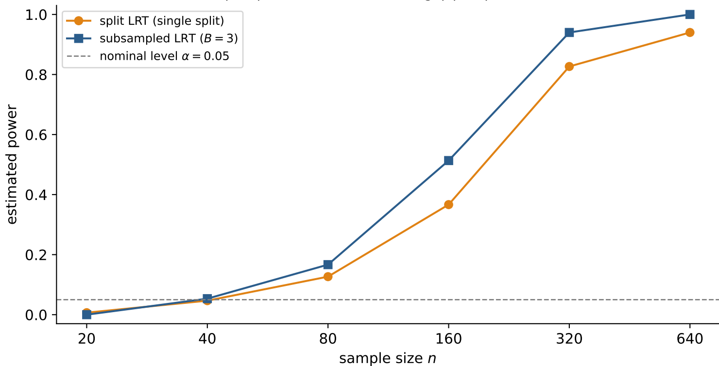
Power of the split/subsampled LR e-value test H_0 : \mu_1 = \mu_2 vs. mixture with true gap \mu_1 - \mu_2 = -2 \times 0.8
