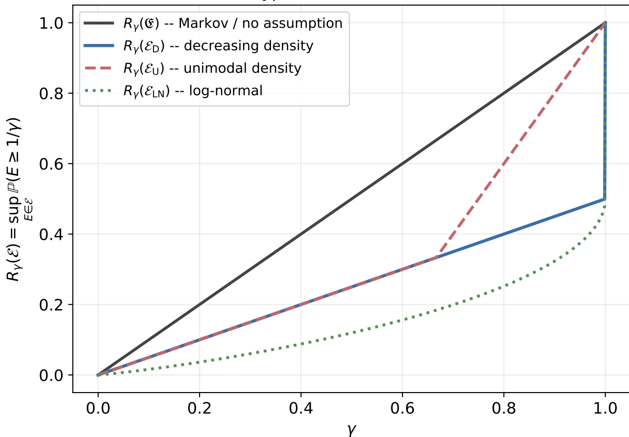
Worst-case type-I error under extra conditions
