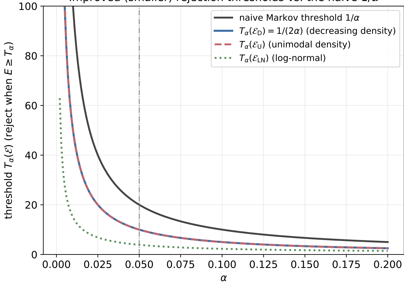
Improved (smaller) rejection thresholds vs. the naive 1/\alpha
