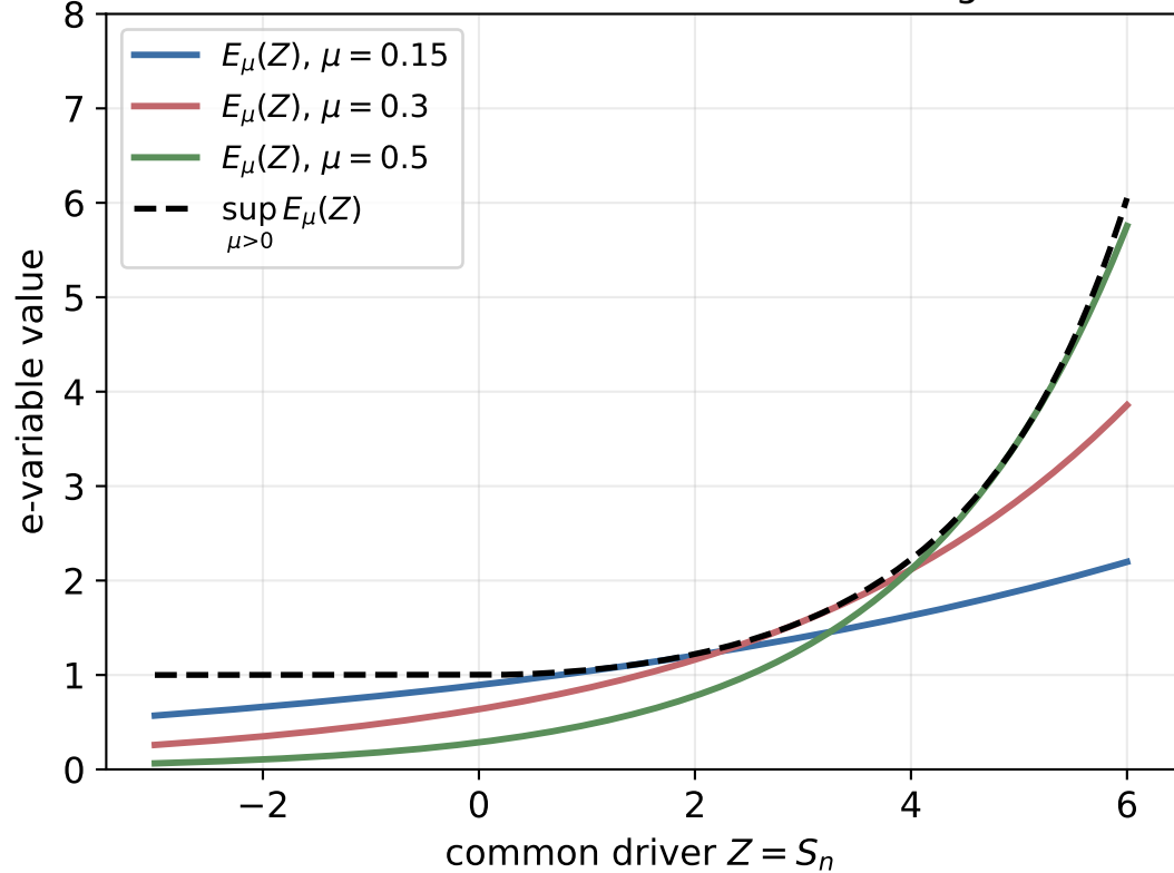
Comonotonic e-variables: all increasing in Z
