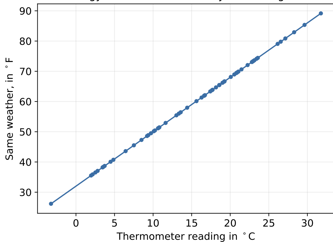
Analogy: comonotonic = always move together
