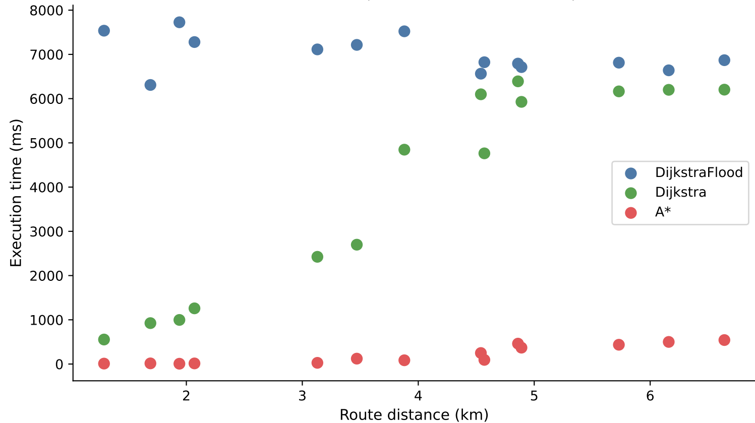
Edinburgh: Execution time vs Route distance A* is 20-100x faster; DijkstraFlood is distance-independent
