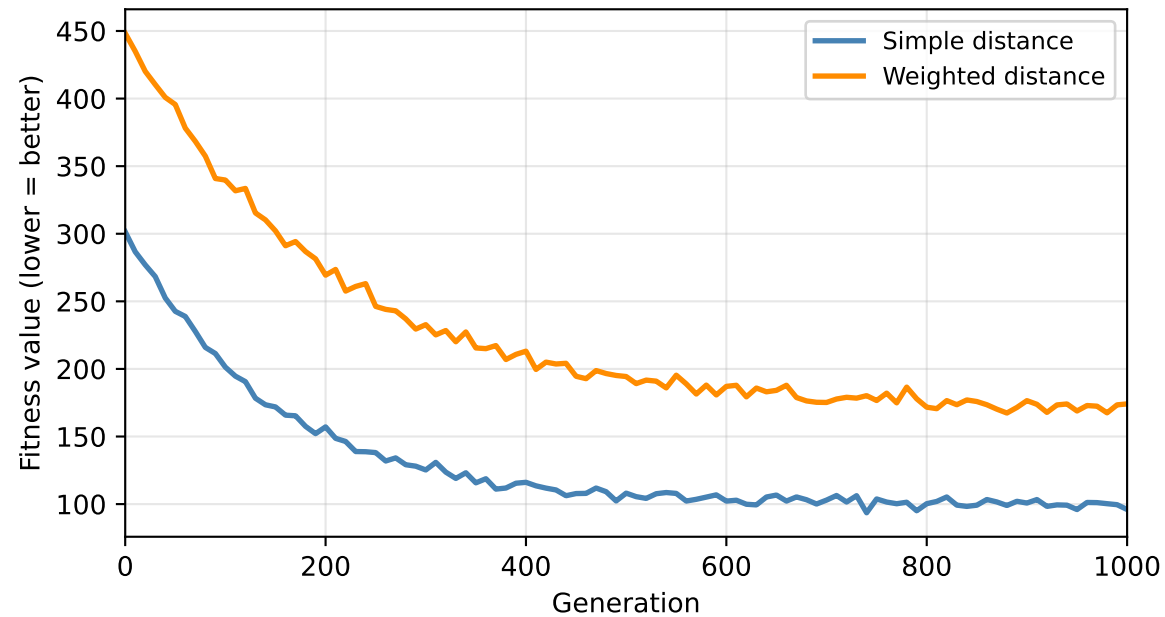
Convergence: Simple vs Weighted Fitness
