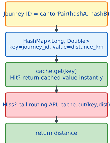
HashMap Cache Architecture (avoids redundant routing API calls)
