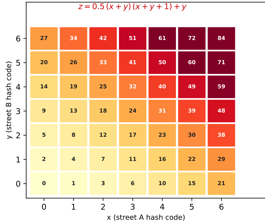
Cantor Pairing: unique key z for each (x, y) pair
