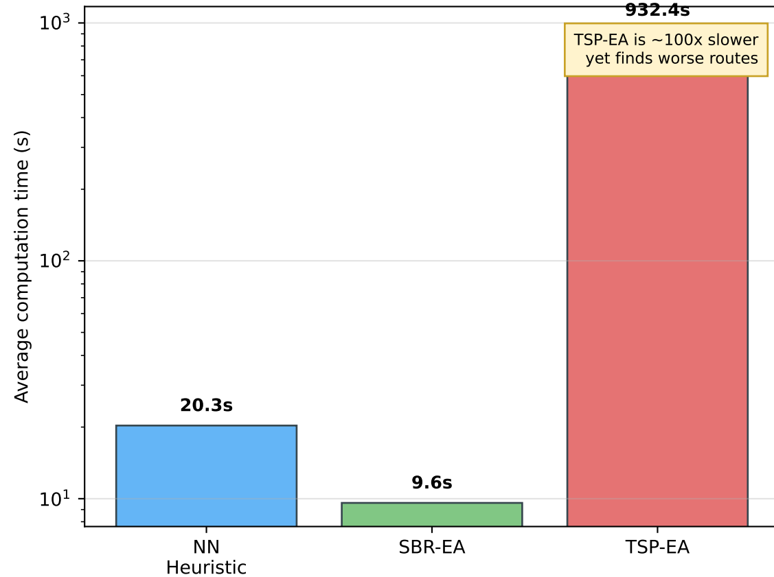
Computation Time Comparison (100,000 evaluations budget)
