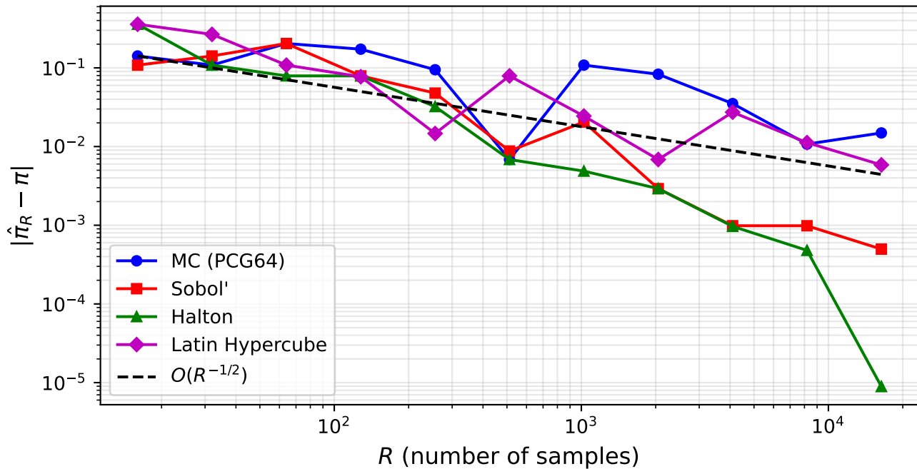
MC vs QMC convergence to \pi
