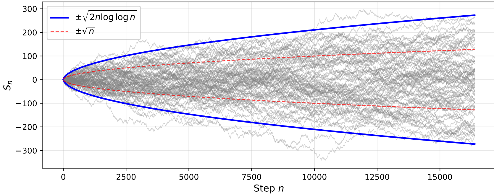
Law of the Iterated Logarithm: 80 trajectories, N = 2^{14}
