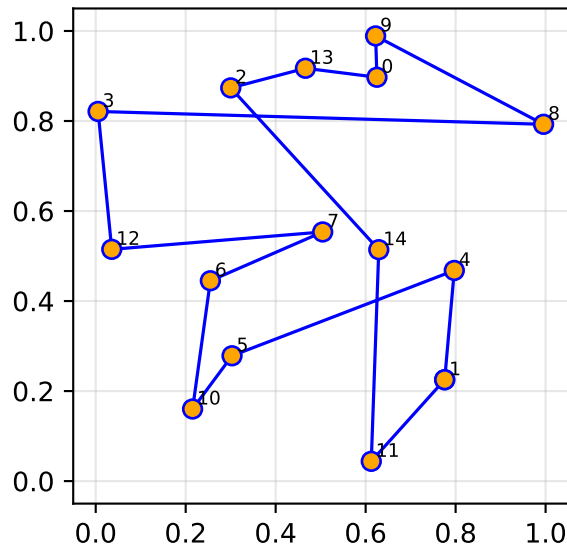
Best of 20,000 random tours (length=5.296)
