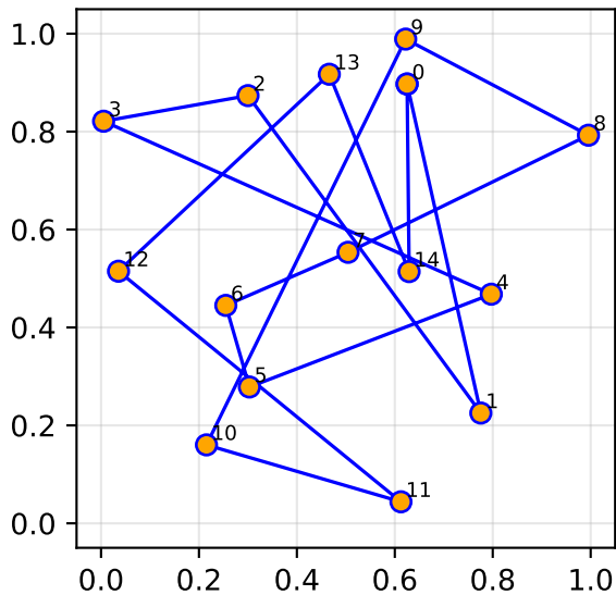
Arbitrary order (no tour)
