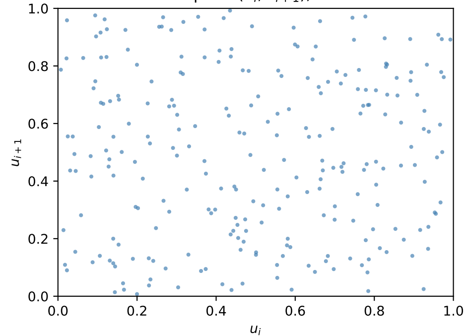
PCG64 pairs (u_i, u_{i+1}) , n = 256
