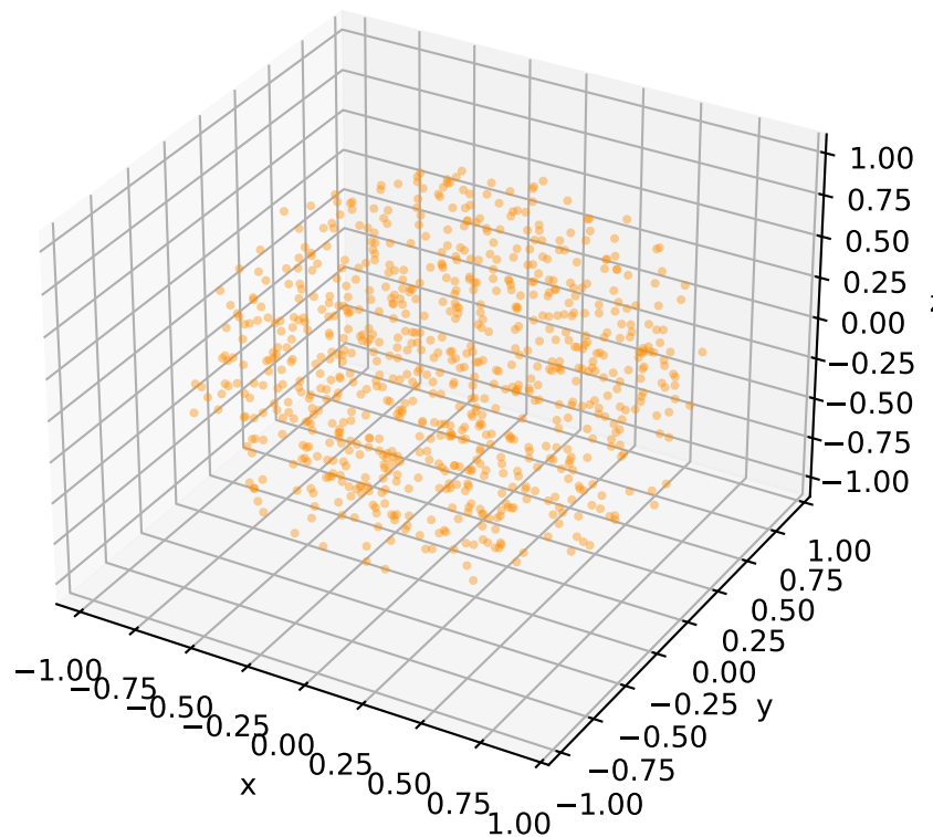
Uniform in B_3 (ball)
