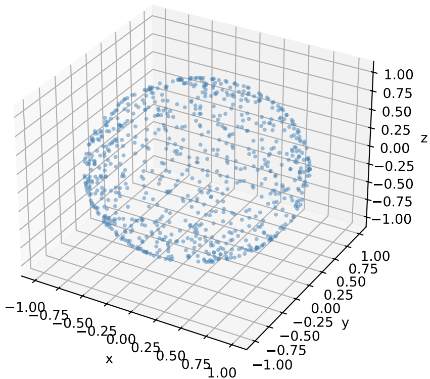
Uniform on S_2 (sphere)
