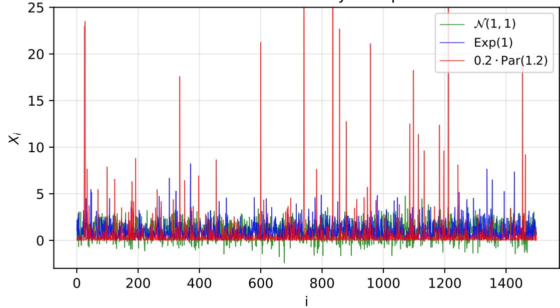
Time series — heavy tail spikes
