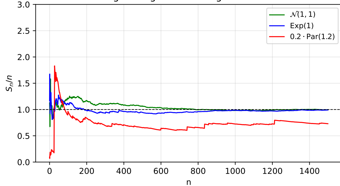
Running averages — convergence to mean 1
