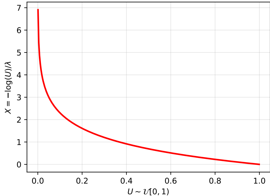
Inverse CDF F^{\leftarrow}(u) = -\log(u)/\lambda
