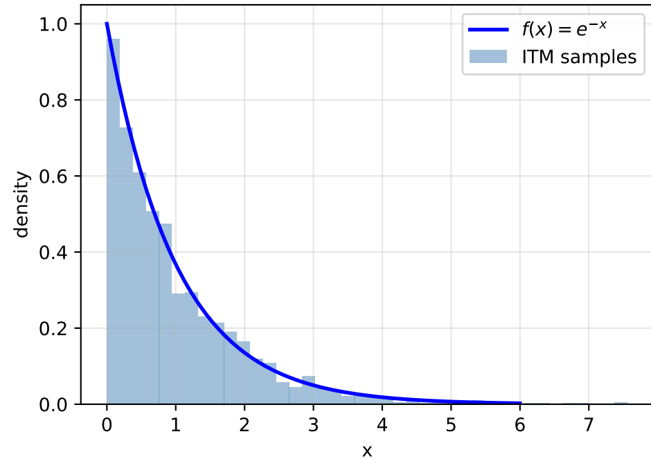
Exponential(1) via ITM
