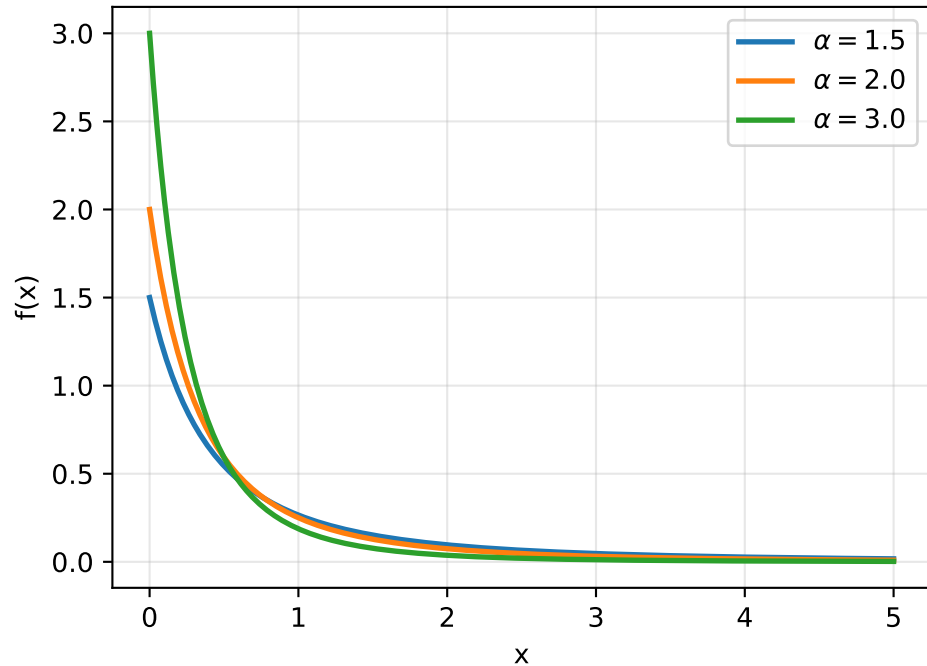
Pareto PDF (heavy tail for small \alpha )
