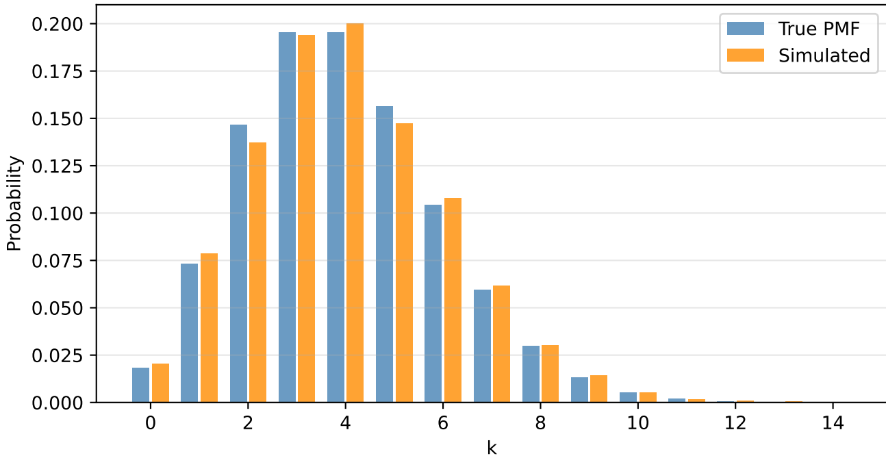
Poisson( \lambda = 4.0 ): renewal-process method
