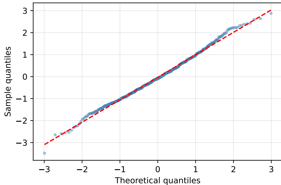
QQ plot: Normal \mathcal{N}(0, 1)
