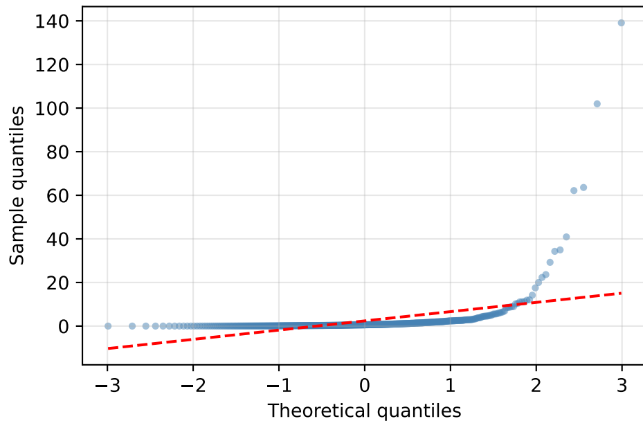
QQ plot: Pareto(1.5) (heavy tail)
