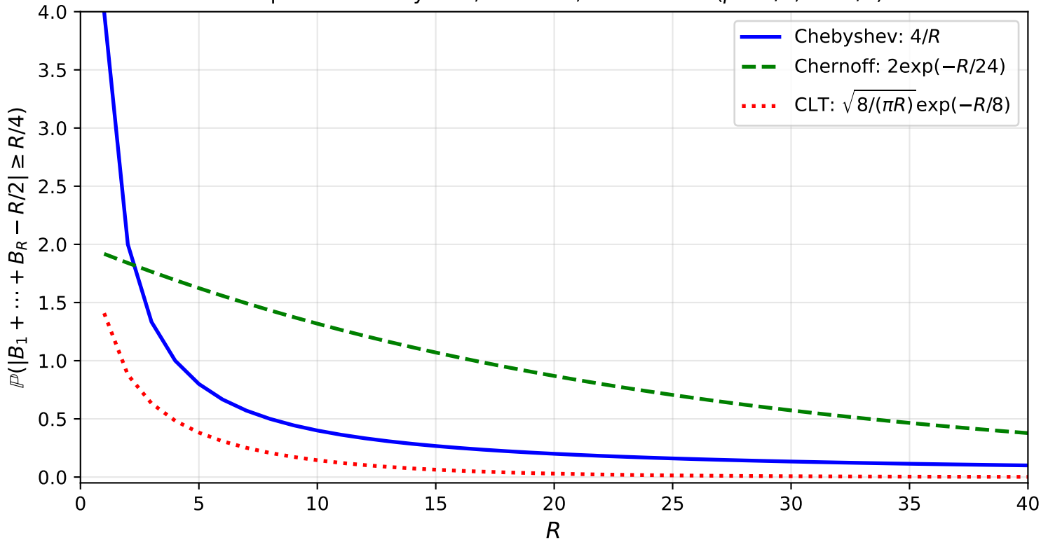
Comparison: Chebyshev, Chernoff, CLT bounds ( p = 1/2 , \varepsilon = 1/2 )
