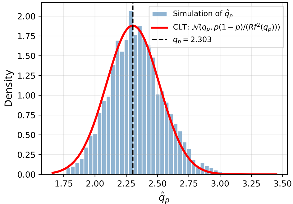
CLT for sample quantile \hat{q}_p
