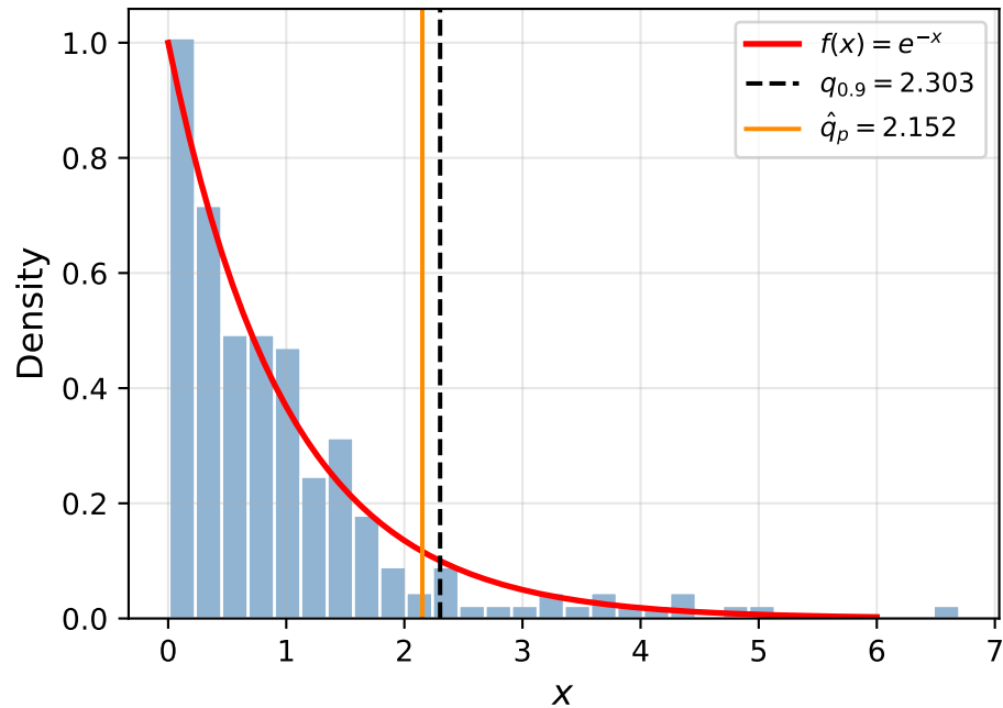
Exp(1) sample ( R = 200 ), 0.9-quantile
