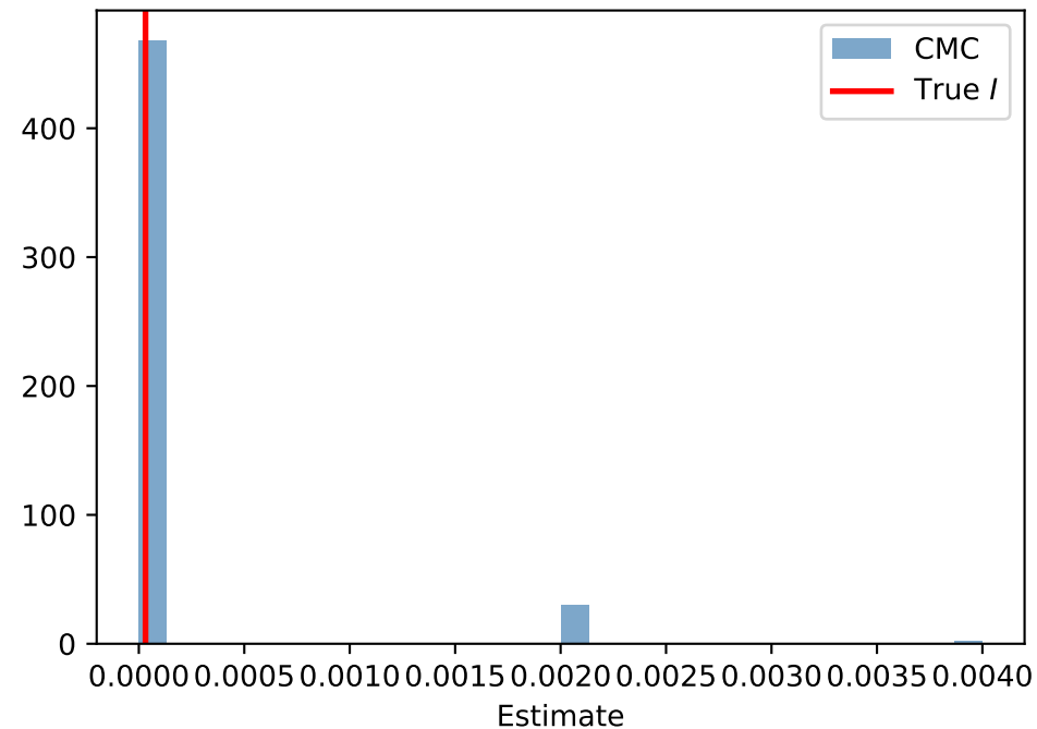
CMC Estimates of P(Z > 4)
