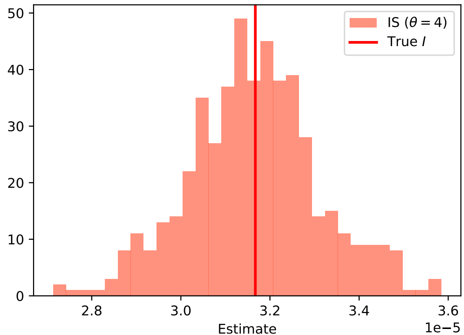
IS Estimates of P(Z > 4)
