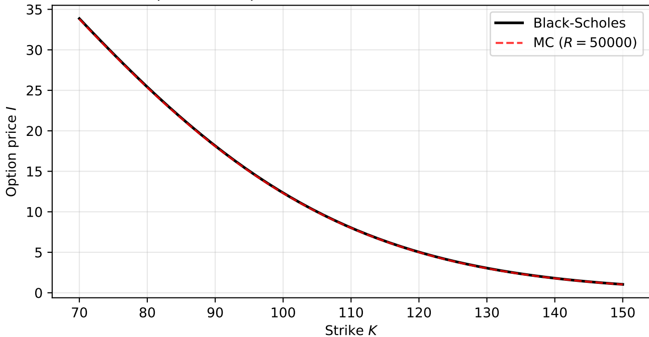
European Call Option Price: Black-Scholes vs Monte Carlo
