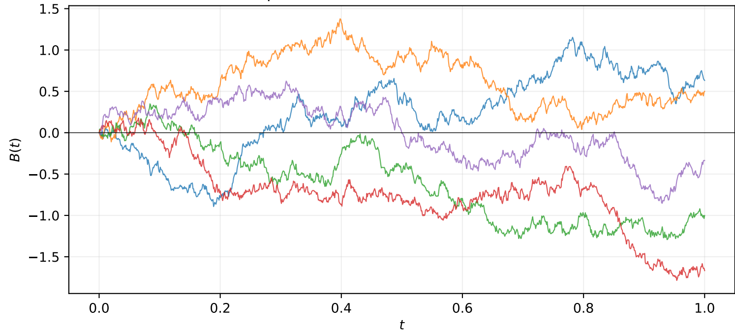
Sample Paths of Standard Brownian Motion
