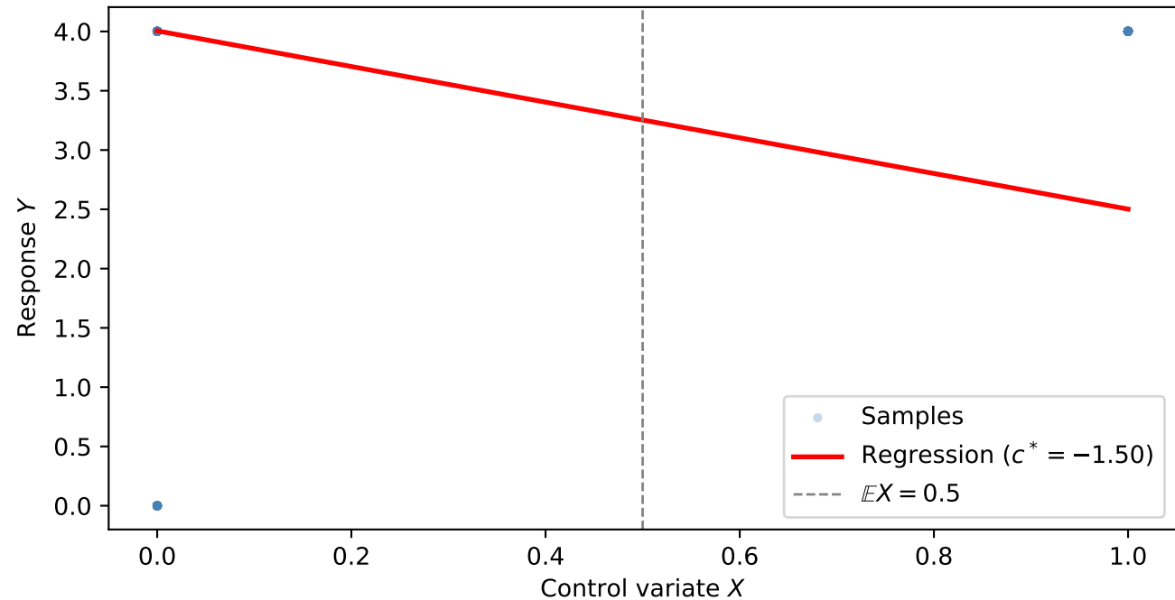
Control Variate Regression ( \pi estimation)
