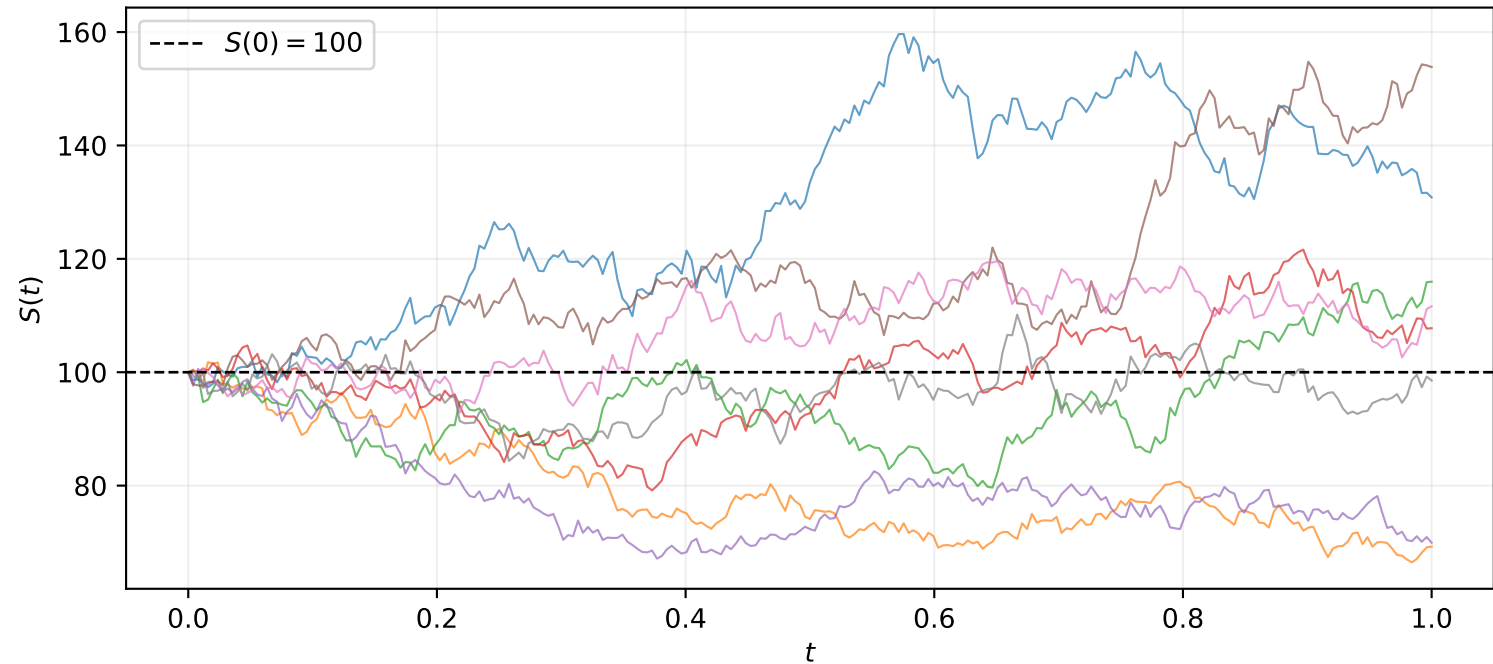
Geometric Brownian Motion Paths ( r = 0.05 , \sigma = 0.25 )
