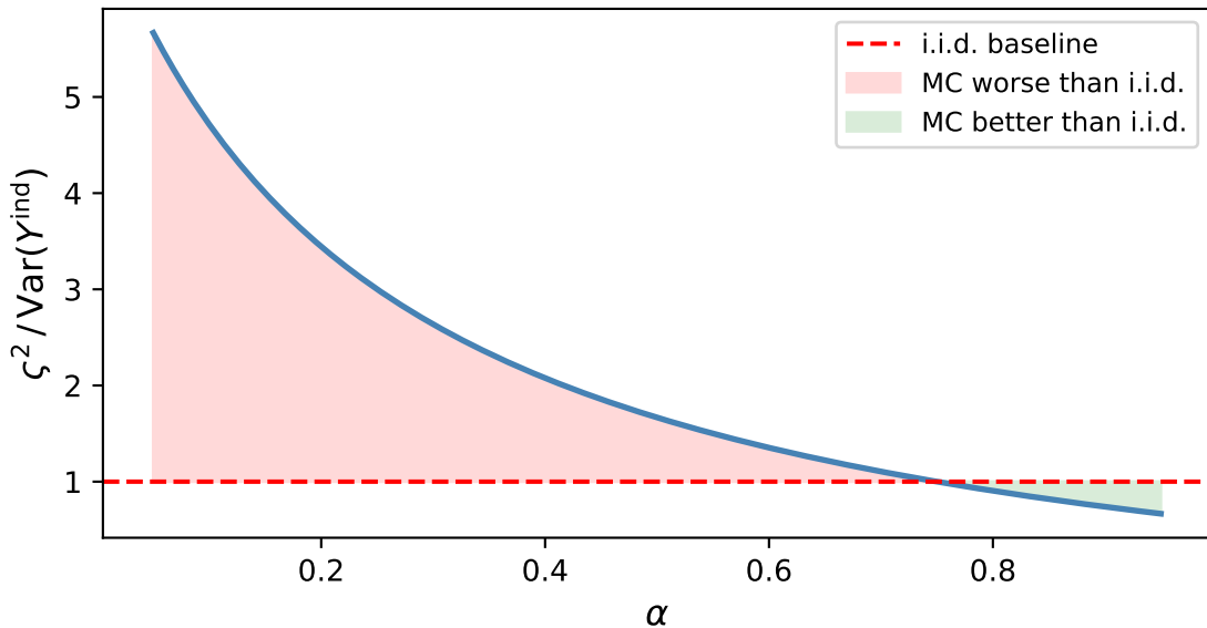
Asymptotic variance ratio ( \beta = 0.25 )
