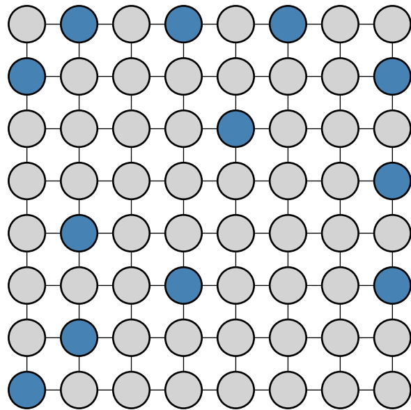
Step 3000 (12 particles)
