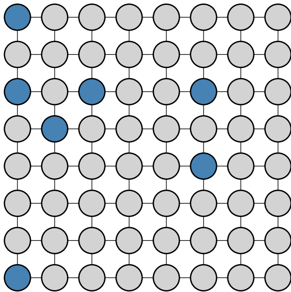
Step 20 (7 particles)
