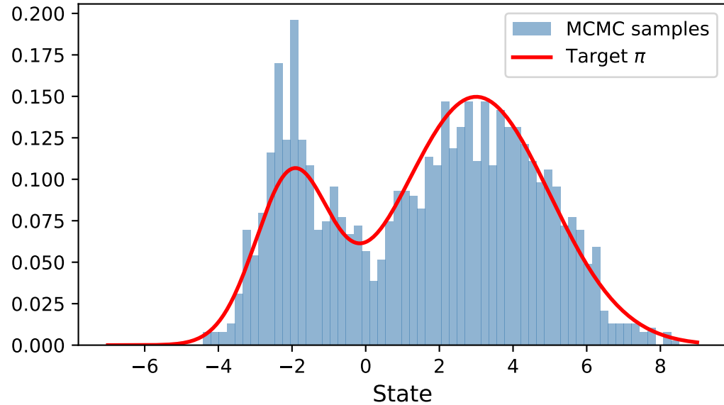
Sample histogram vs target
