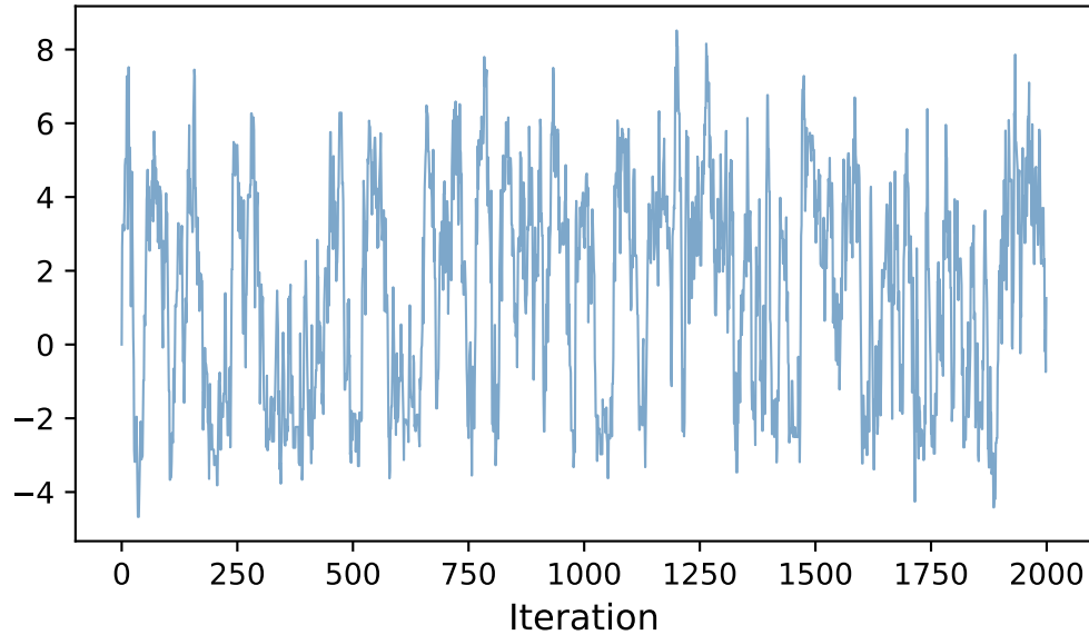
MH trace (acceptance rate 79.8%)
