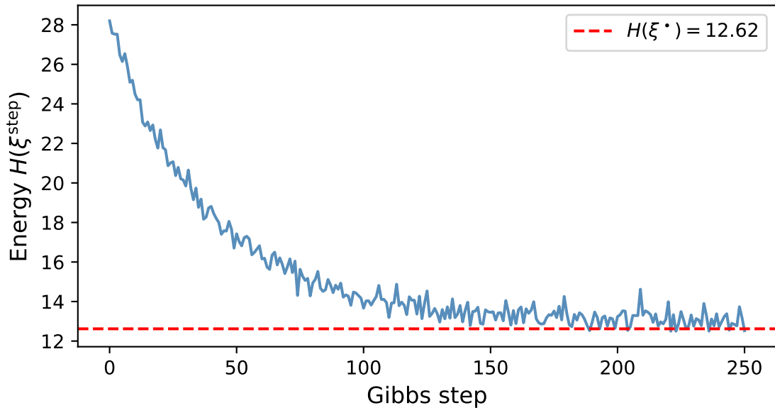
Motif finding: energy during Gibbs sampling
