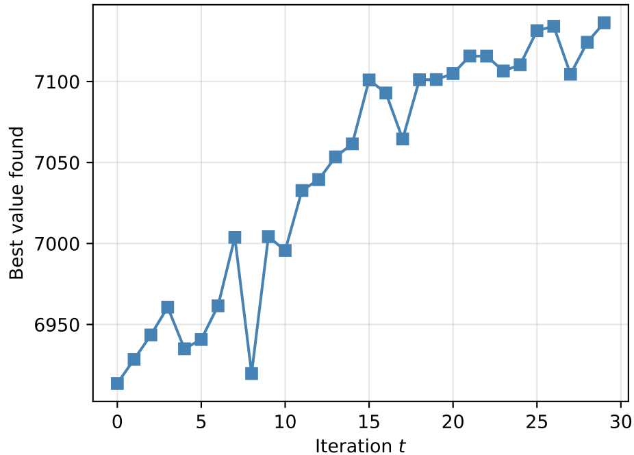
CE: best knapsack value vs iteration
