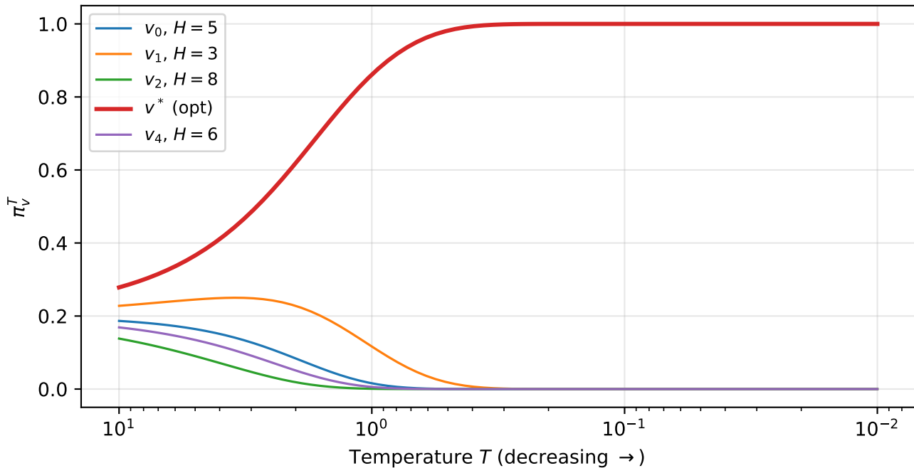
Boltzmann mass concentrates on optimum as T \searrow 0
