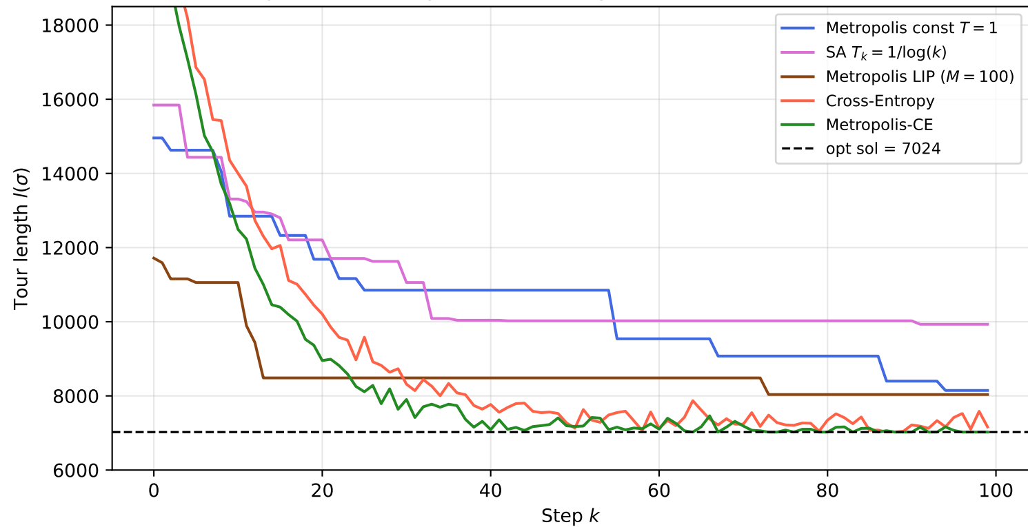
Fig 7.4 - 100 steps of various algorithms for TSP (13 cities)
