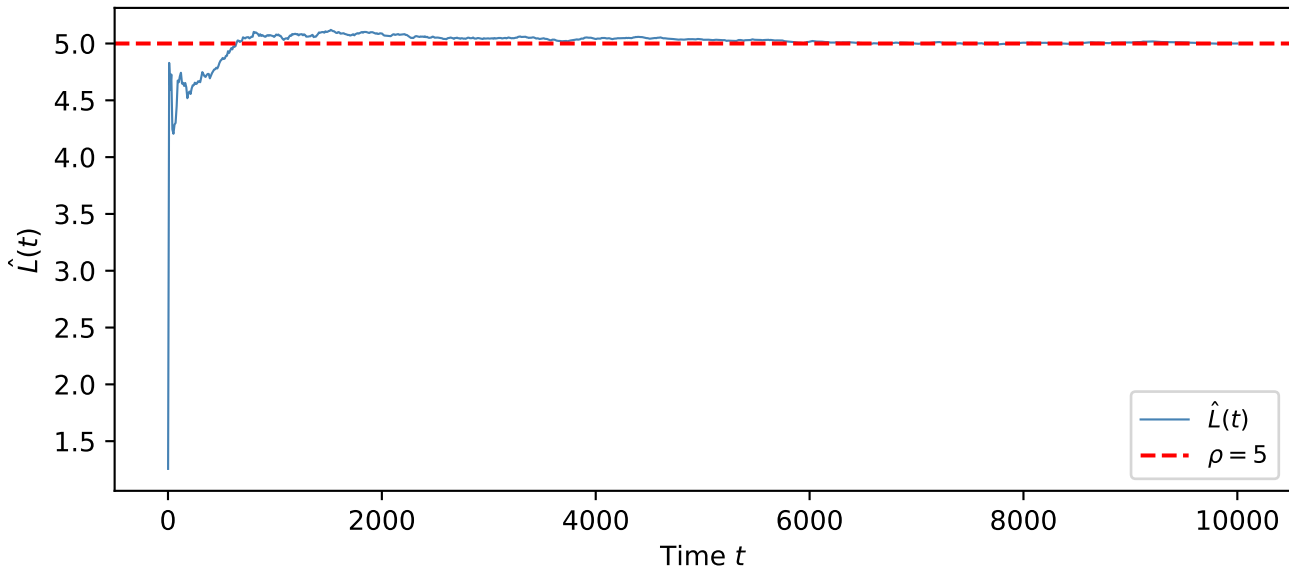
M/M/ \infty Queue: Running Mean ( \lambda = 5 , \mu = 1 )
