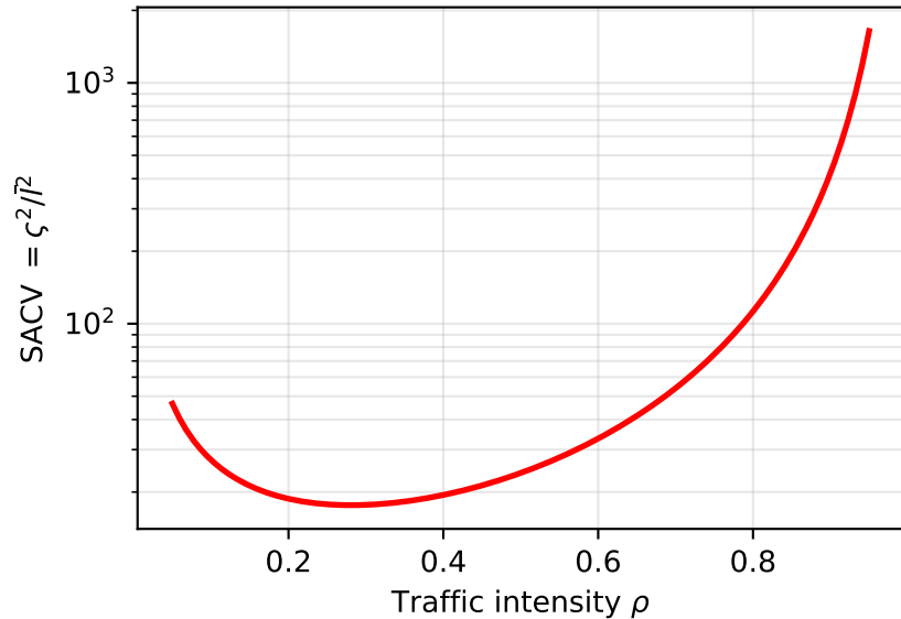
Squared Asymptotic Coefficient of Variation
