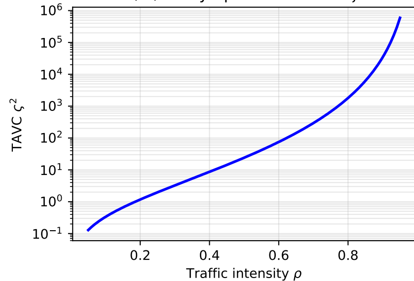
M/M/1: Asymptotic Variance \zeta^2
